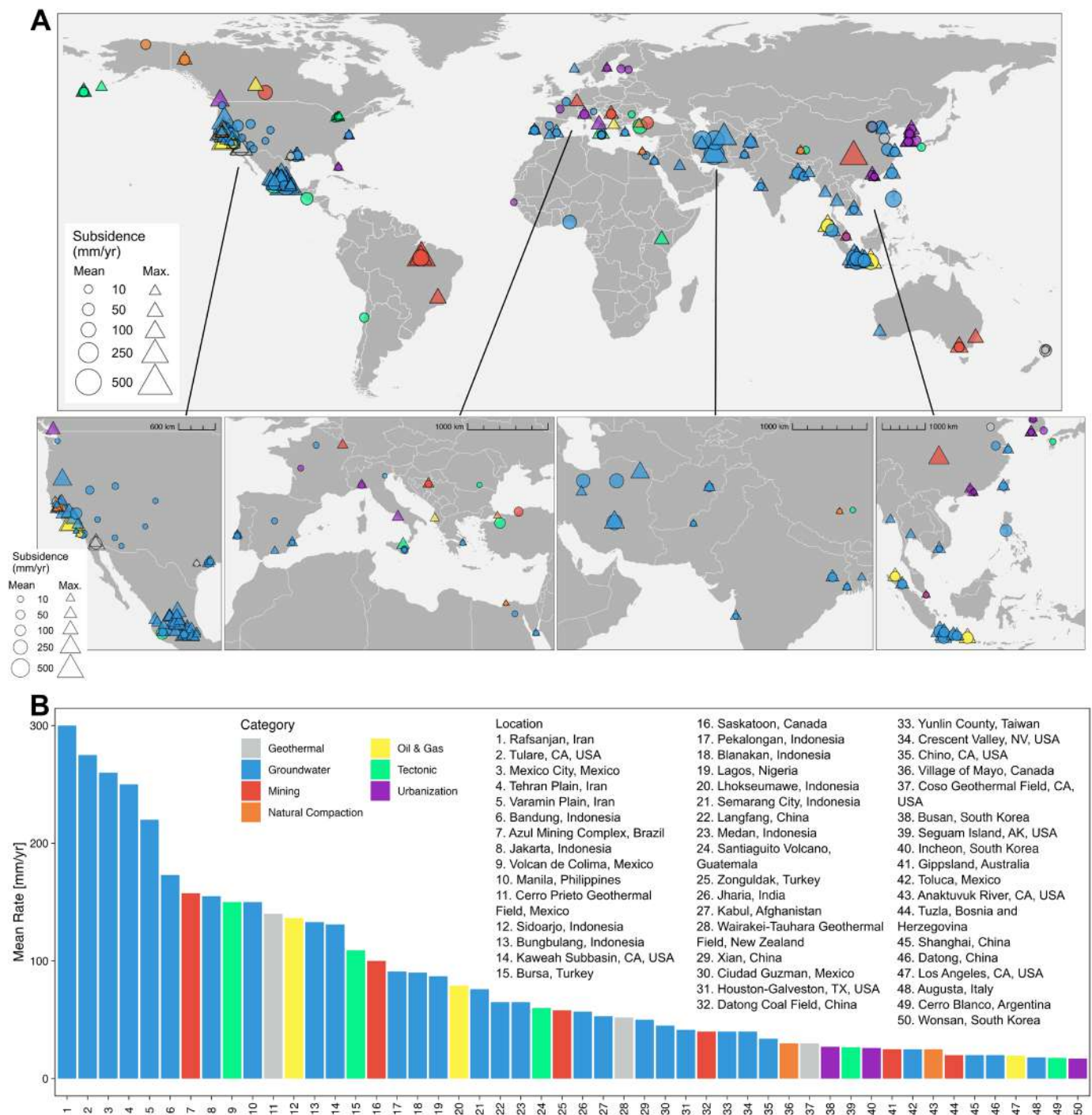
Figure 6. Reported land subsidence rates and drivers across the globe. (A) Global map of main land subsidence drivers (colors) with mean (circles) and maximum (triangles) rates (shape sizes). (B) The primary causes of land subsidence rates at each location. Image source: Huning et al. (2024), Reviews of Geophysics.
